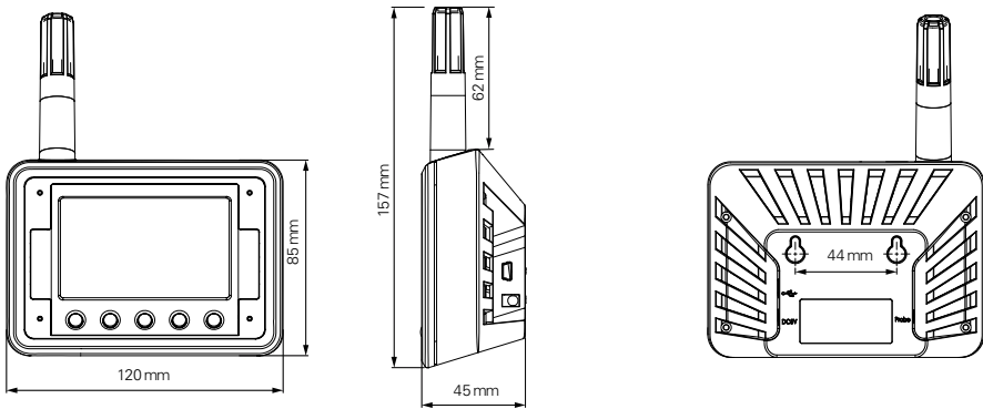
Dimensions CL11
